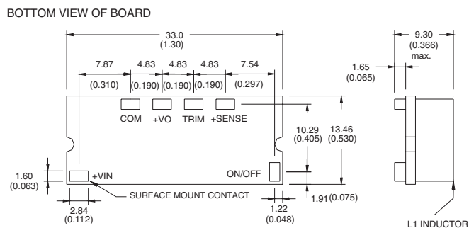
Figure 16 VPOL16A-12-SMT Mechanical Outline Diagram
